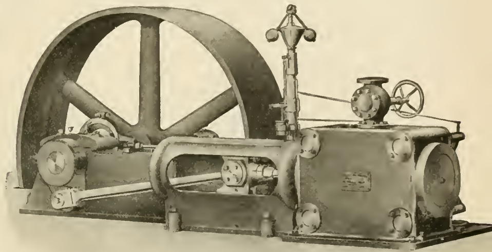
NEW STANDARD REYNOLDS-CORLISS ENGINE—ALLIS-CHALMERS CO.
